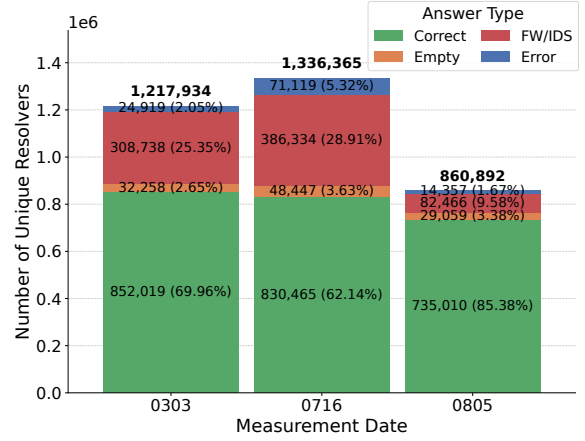
Figure 5: Illustration of correctness.
