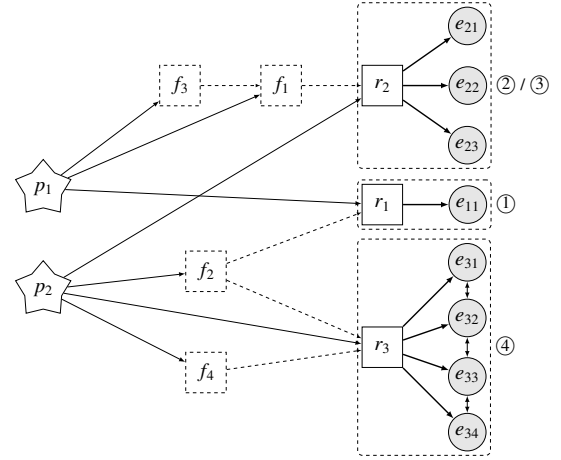
Figure 1: ODNS Architecture. Stars are probes, rectangles are recursors, circles are egresses, and dashed rectangles are forwarders. Solid lines are direct requests; dashed lines denote forwarded requests. Recursor types defined in Section 3.2.1 are labeled ① to ④.
