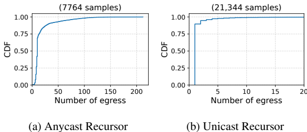
Figure 9: Egress Set Size Distribution
